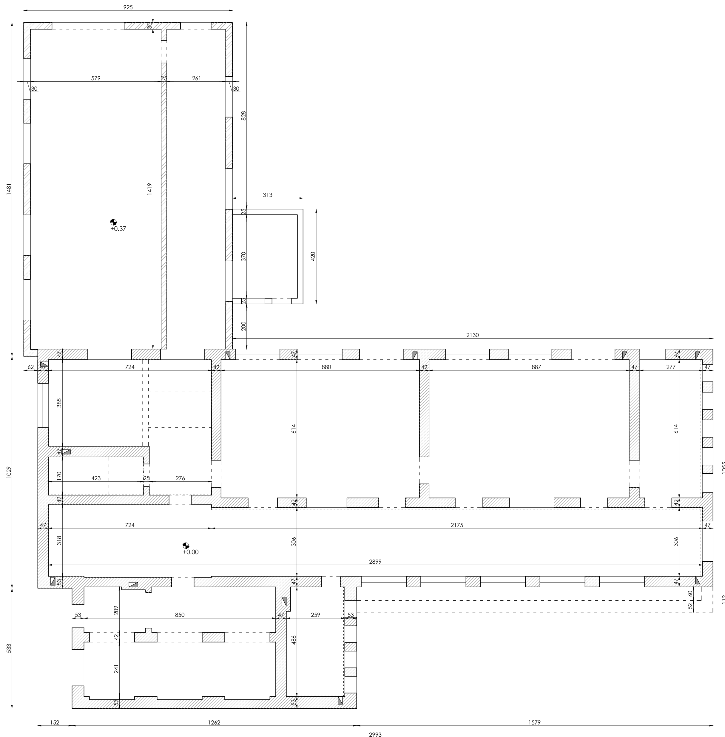
PIANTA MURATURE PIANO SEMINTERRATO
